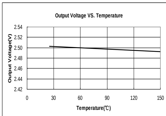
QN6118A25B3G ( V_{IN}=V_{OUT}+1.2V , I_{OUT}=10mA )
