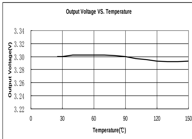
QN6118A33B3G ( V_{IN}=V_{OUT}+1.2V , I_{OUT}=10mA )
